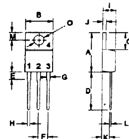
TO-220
