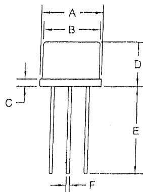
TO-39 CASE - MECHANICAL OUTLINE
