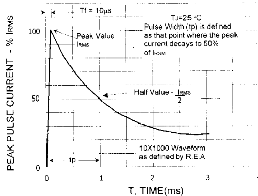
FIG. 3 - PULSE WAVEFORM
